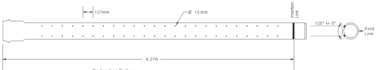
Perforation Pattern: 2 rows of 13 mm diameter holes 127mm spacing centre to centre 120° +/- 5° apart
