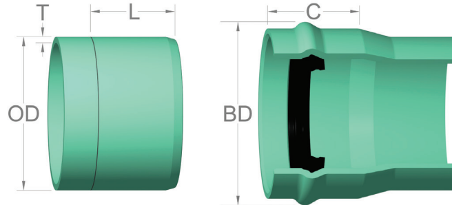
GASKETED SEWER PIPE DIMENSIONS &amp; PERFORMANCE
