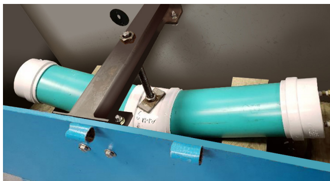
Figure 3 – Example of Angular Joint Deflection Setup for Pressure and Vacuum Tests for standard sewer fitting
