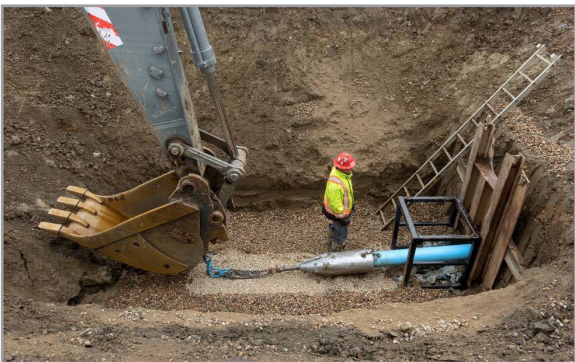
Figure 10. Removal of Bursting Head from Machine Pit
