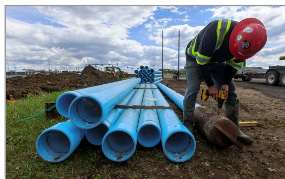
Figure 5. Attachment of Expander Head to the Pipe
