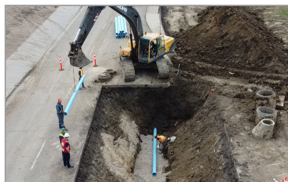
Figure 4. Aerial View of Insertion Pit – 62 nd Avenue
