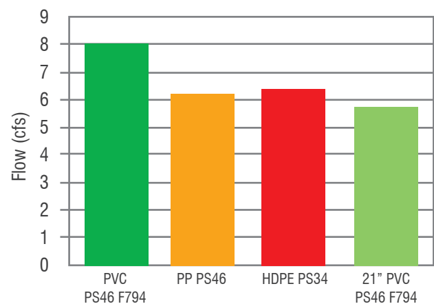
FIGURE A.11 : 24" PROFILE-WALL PVC GRAVITY PIPE FLOW COMPARISONS WITH EQUIVALENT SLOPE
