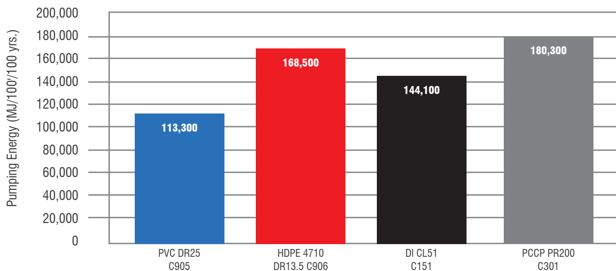
FIGURE A.19 : 24" PVC DR25 EQUIVALENT PIPES 100-YEAR PUMPING ENERGY
