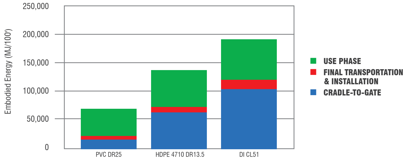
FIGURE 12.2 : TOTAL 100-YEAR EMBODIED ENERGY FOR 8" PVC DR25 EQUIVALENT PRESSURE PIPES
