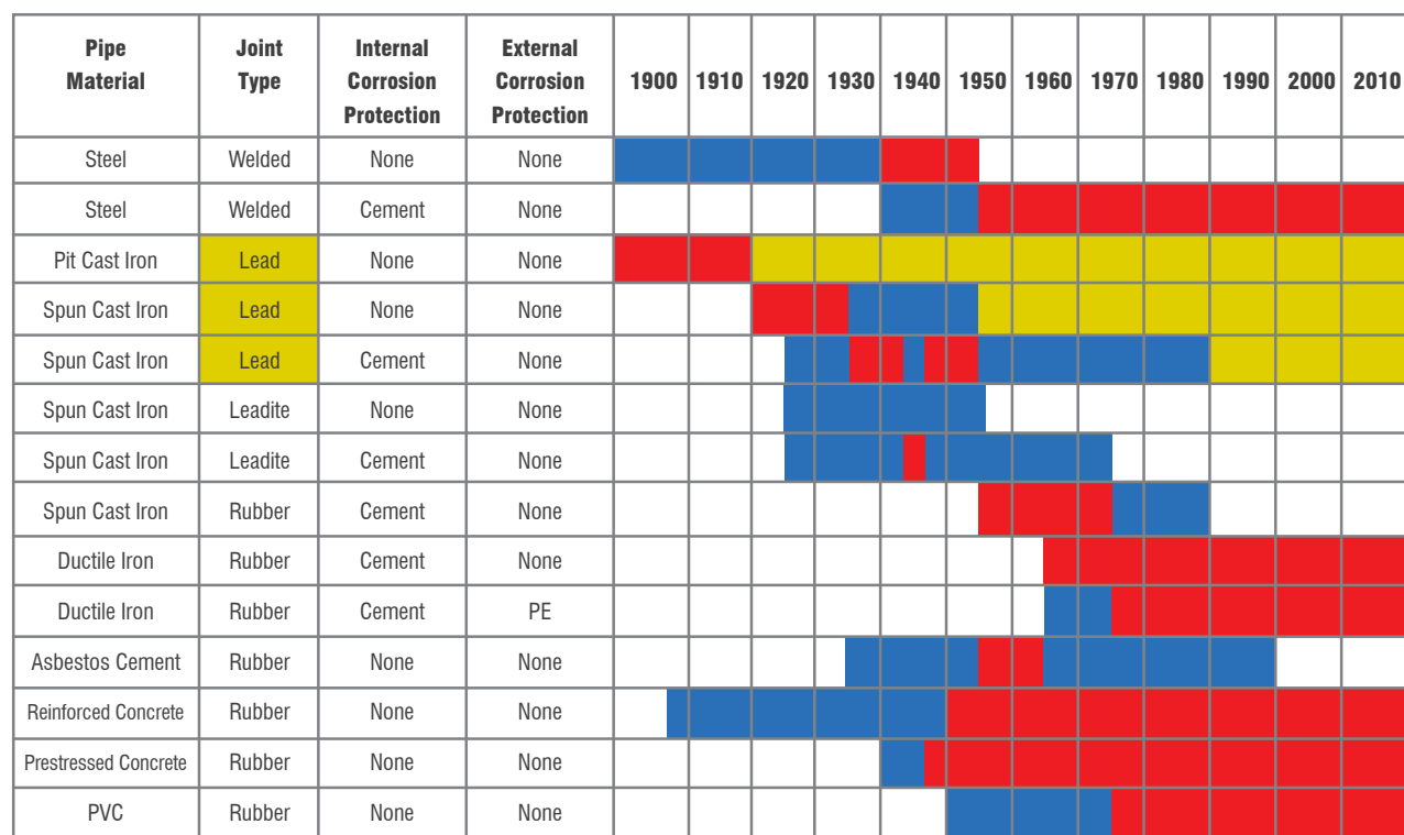
FIGURE 8.3 : TIMELINE OF PIPE TECHNOLOGY IN THE U.S. IN THE 20 TH CENTURY
