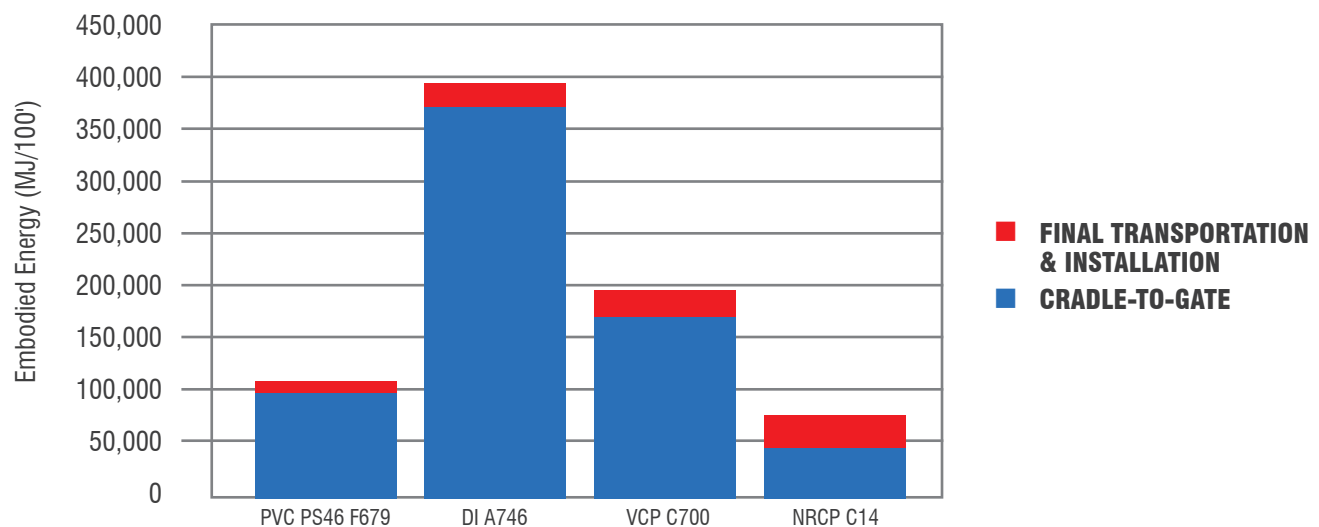
FIGURE 12.8 : TOTAL 100-YEAR EMBODIED ENERGY FOR 24" PVC PS46 F679 SOLID-WALL EQUIVALENT GRAVITY PIPES
