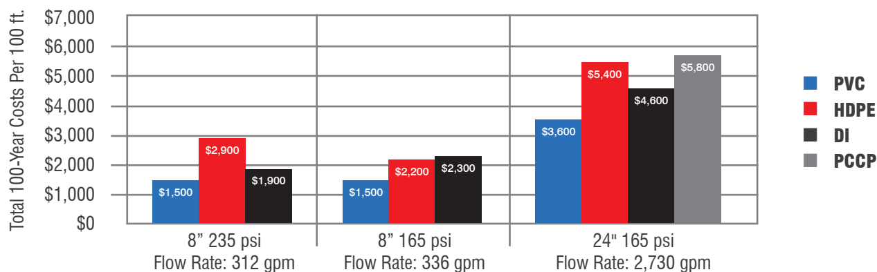
FIGURE A.4 : TOTAL 100-YEAR PUMPING ENERGY COSTS PER 100 FEET OF PIPE
