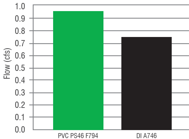
FIGURE A.10 : 8" PROFILE-WALL PVC GRAVITY PIPE FLOW COMPARISONS WITH EQUIVALENT SLOPE
