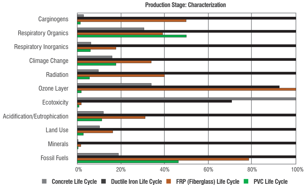
FIGURE A.27 : CHARACTERIZATION GRAPH FOR LIFE CYCLE COMPARISON FOR ALL PIPING MATERIALS
