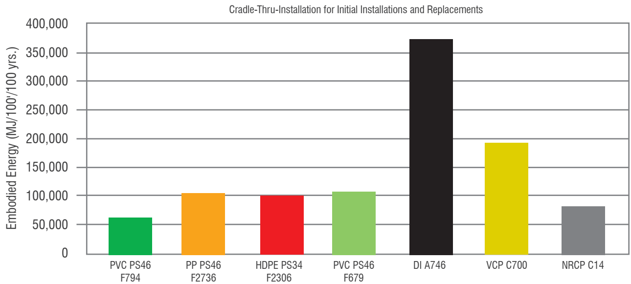
FIGURE A.8 : TOTAL 100-YEAR EMBODIED ENERGY FOR 24" GRAVITY PIPE PRODUCTS
