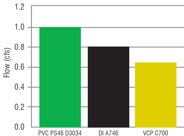
FIGURE A.12 : 8" SOLID-WALL PVC GRAVITY PIPE FLOW COMPARISONS WITH EQUIVALENT SLOPE
