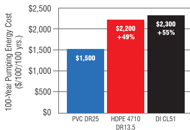
FIGURE A.15 : PUMPING ENERGY COST OF 8" PVC DR25 EQUIVALENT PIPES OVER A 100-YEAR LIFE CYCLE
