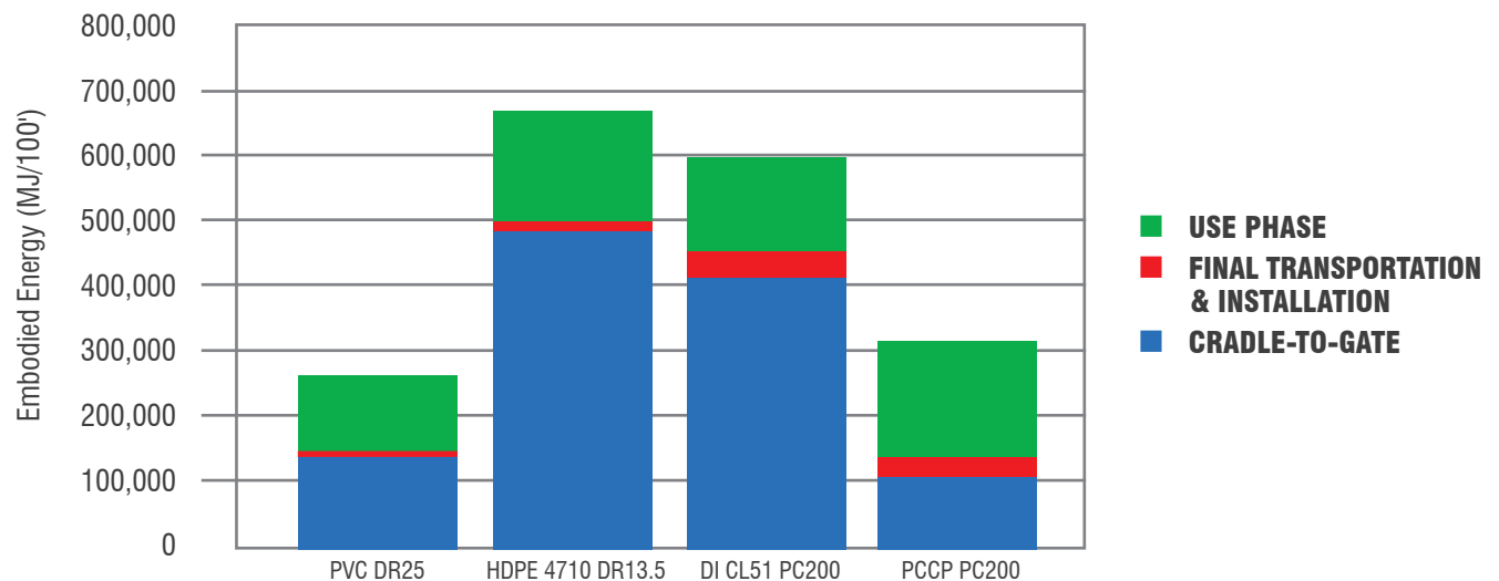
FIGURE 12.3 : TOTAL 100-YEAR EMBODIED ENERGY FOR 24" PVC DR25 EQUIVALENT PRESSURE PIPES
