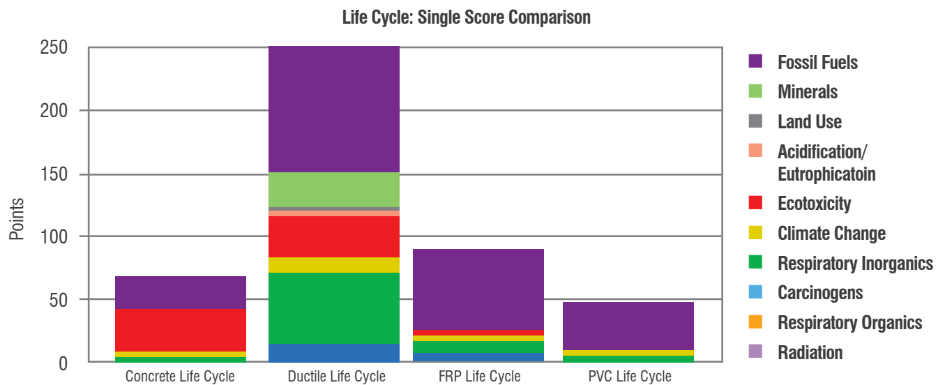
FIGURE A.28 : SINGLE SCORE GRAPH FOR LIFE CYCLE COMPARISON FOR ALL PIPING MATERIALS
