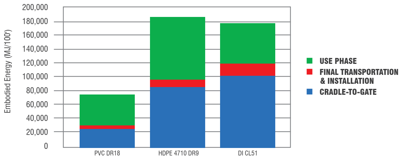
FIGURE 12.1 : TOTAL 100-YEAR EMBODIED ENERGY FOR 8" PVC DR18 EQUIVALENT PRESSURE PIPES
