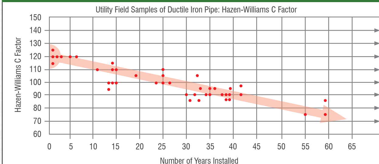
FIGURE 8.5 : FIELD SAMPLES SHOWING DECLINING C FACTOR FOR DI PIPE
