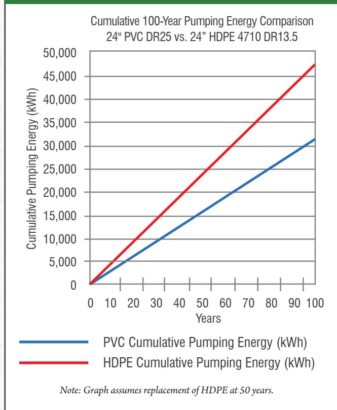
FIGURE 9.6 : COMPARISON OF CUMULATIVE 100-YEAR PUMPING ENERGY FOR 24" PVC AND HDPE PIPE
