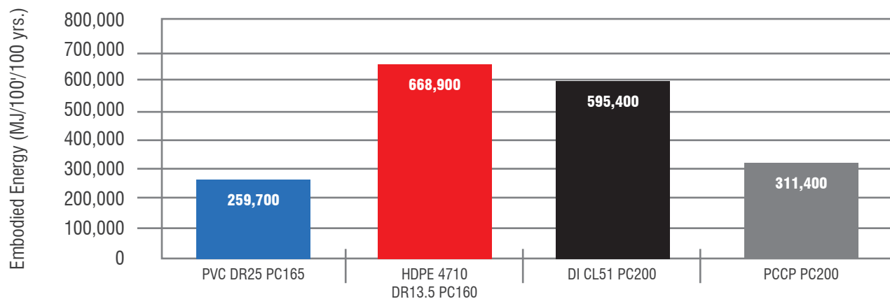
FIGURE A.7 : 24" PVC DR25 EQUIVALENT PIPES: 100-YEAR TOTAL EMBODIED ENERGY
