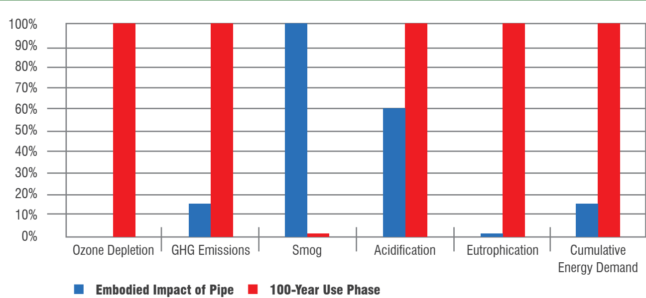
FIGURE 7.1 : ENVIRONMENTAL IMPACTS OF THE USE PHASE OF 8” PVC DR25 PC165 C900 PIPE VS. EMBODIED IMPACTS OF THE PIPE
