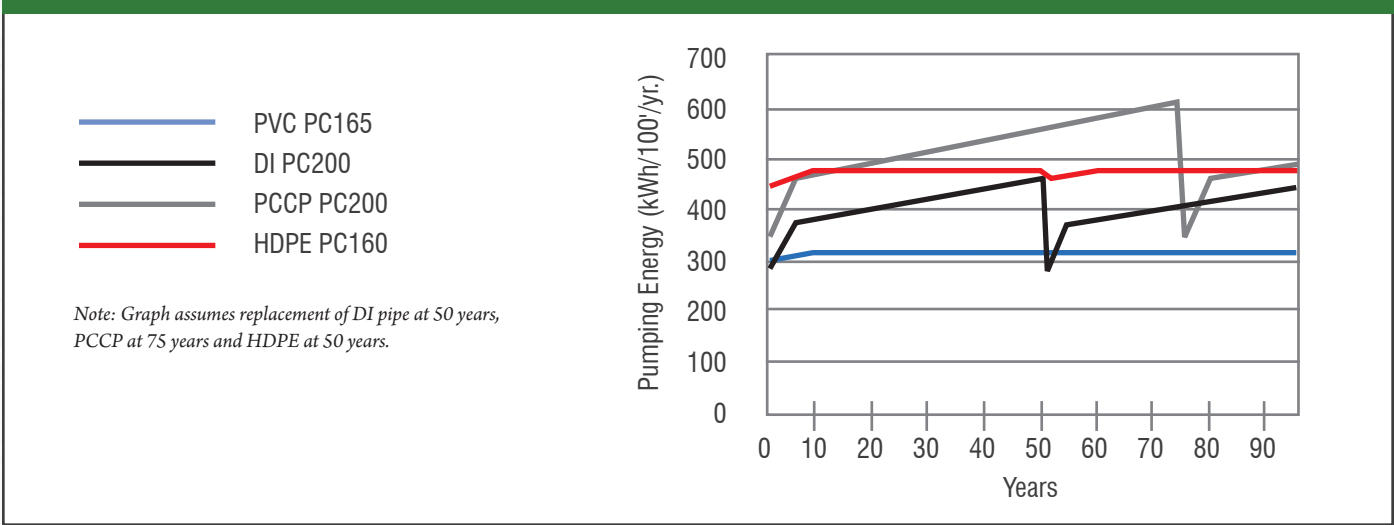
FIGURE 8.4 : ANNUAL PUMPING ENERGY COMPARISONS FOR 24" PIPES
