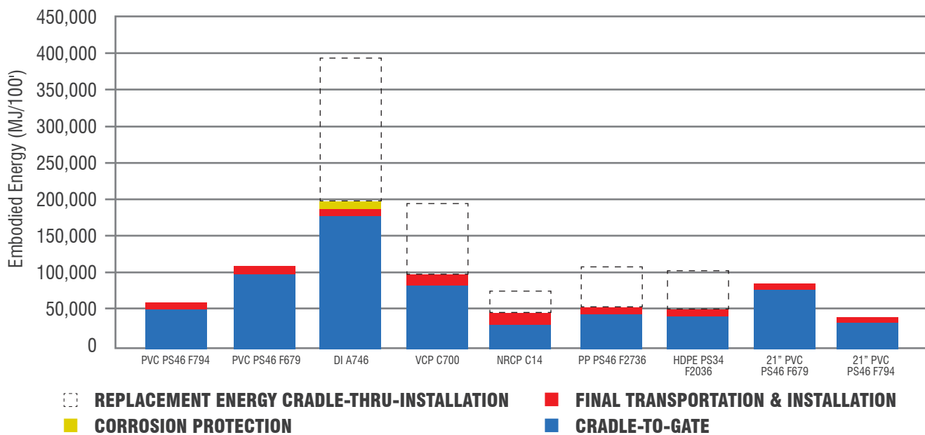
FIGURE 12.10 : TOTAL 100-YEAR EMBODIED ENERGY FOR 24" PVC PS46 SOLID-WALL & PROFILE-WALL EQUIVALENT GRAVITY PIPES
